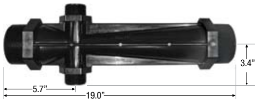
Dimensions for 3090-PVDF
