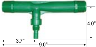
Dimensions for ISO 885X-02-GRPP thru ISO 1078-02-GRPP
