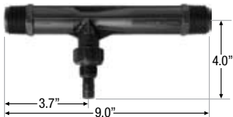
Dimensions for 878-02-PVDF thru 1078-02-PVDF
