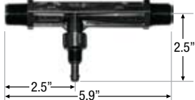
Dimensions for 384-PP thru 584C-PP
