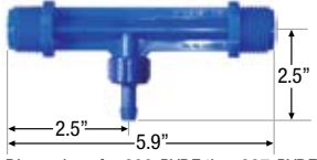
Dimensions for 283-PVDF thru 287-PVDF
