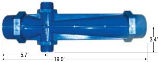
Dimensions for ISO 3090-PVDF
